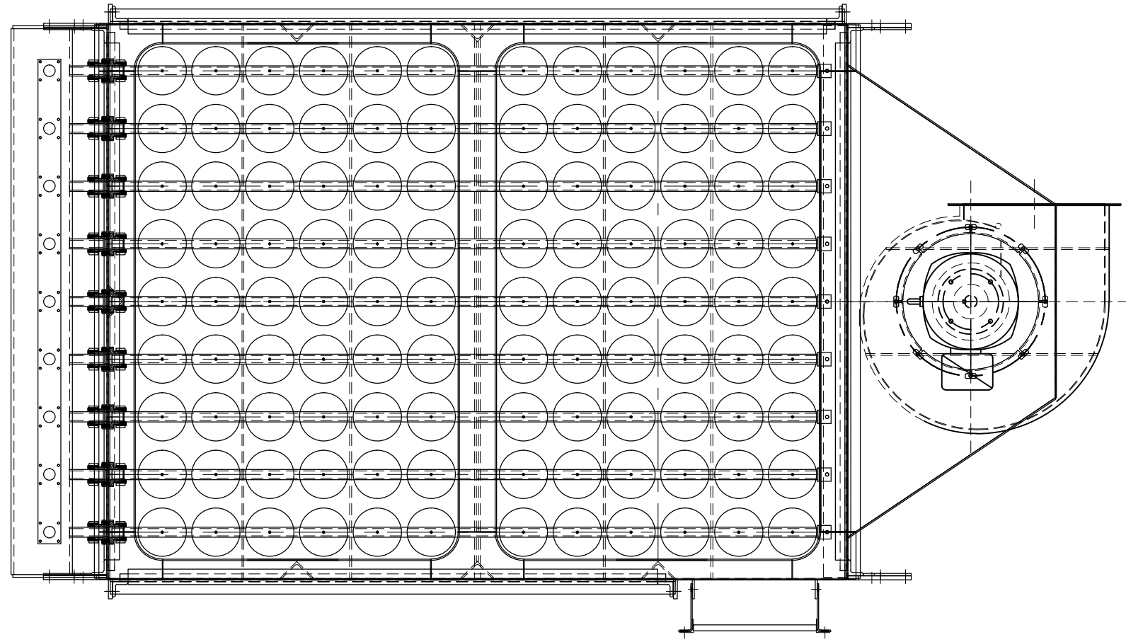
PLAN VIEW
